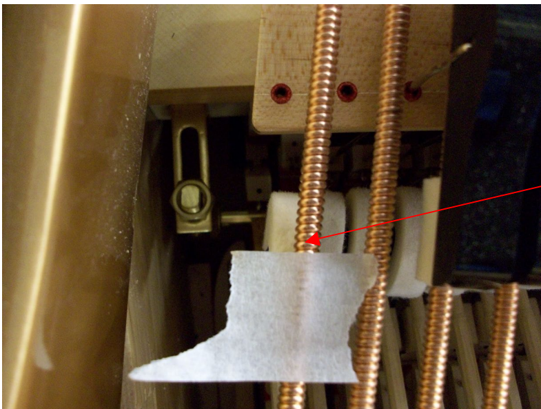
Fig. 18 Edge of tape locating note one strike point
